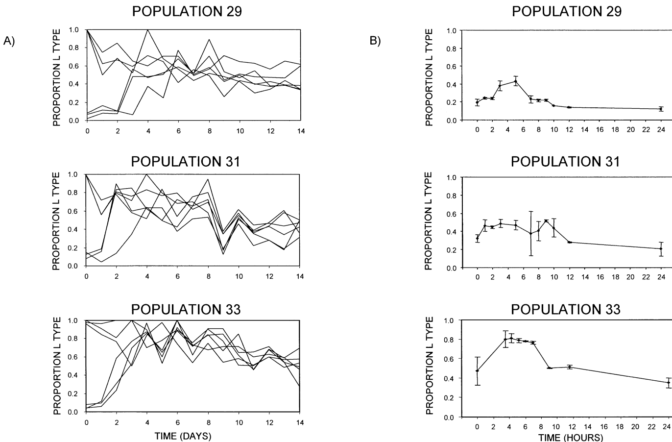
FIG. 6. (A) Results from mutual invasion experiments for populations 29, 31, and 33. The frequency of L types is measured daily for 14 days of serial transfer in 50% acetate plus 50% glucose starting with about 99% L and with 10% L. Each line is a replicate assay. In all cases, the frequency of L types equilibrates at an intermediate level, showing that both L and S types can increase from frequencies. (B) The frequency of a single L strain growing with a single S strain over 24 h for populations 29, 31, and 33. The two strains were grown together for at least three days to reach a stable frequency. Proportions are estimated from plate counts at each time point; error bars represent 95% confidence intervals assuming an underlying normal distribution.
